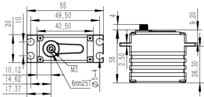
6mm25T Output Shaft Spline
