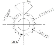
15T 4mm Output Shaft Spline
